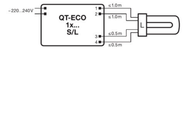
Wiring diagram
