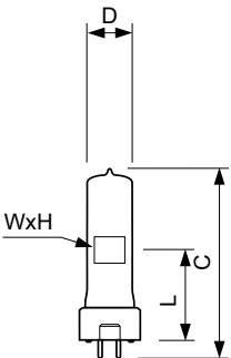
6995I/BP 1000W GY9.5 240V
